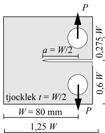
c) Compact Tension (CT) provstav
